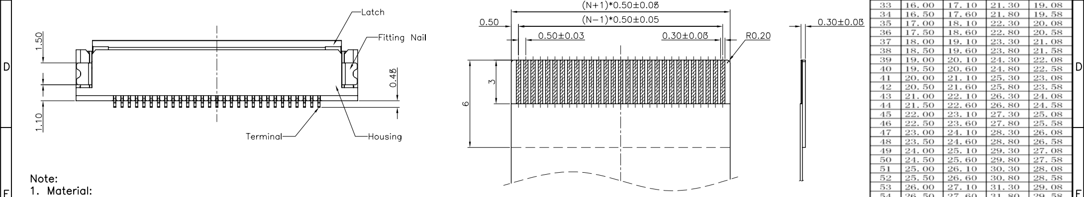
RECOMMENDED FPC/FFC DIMENSION
